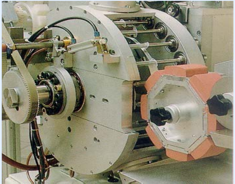
Syringe printing machine
