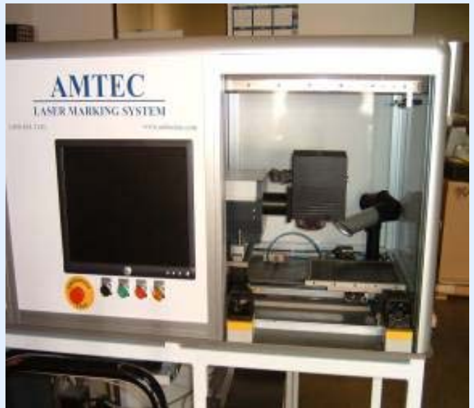
Laser Marker with X-Y stage and Fume Extractor
